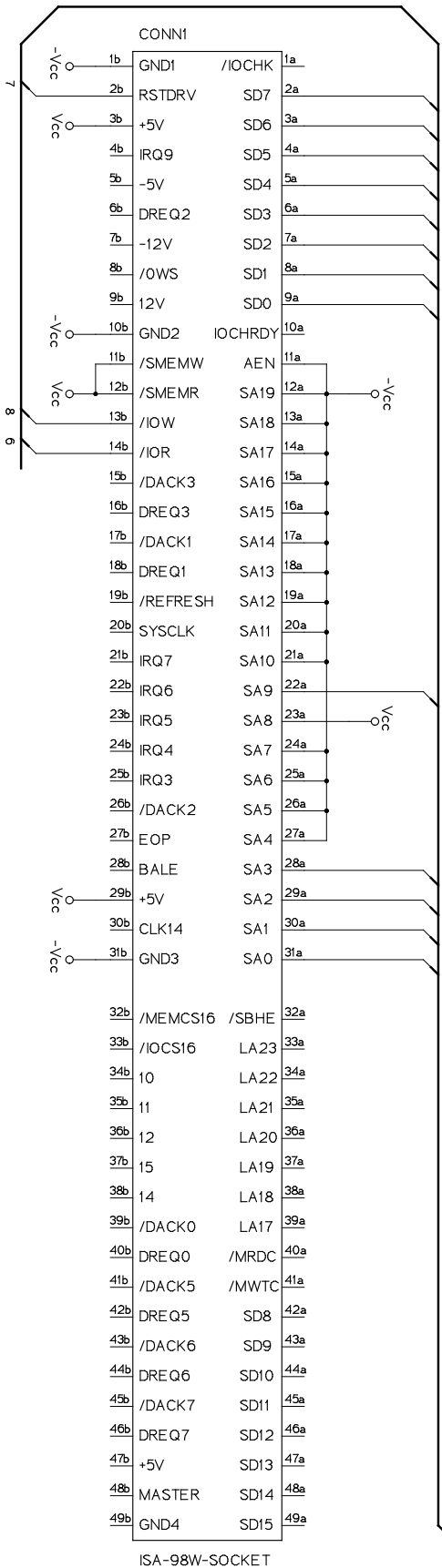
ISA-98W-SOCKET
